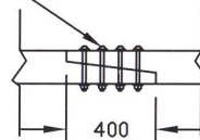
WHEEL GUARD SPLICE
